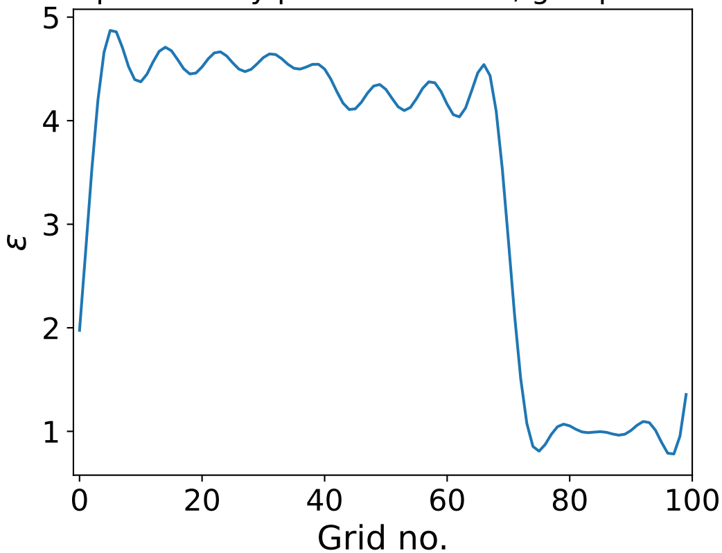
GRCWA permittivity profile. n_G = 25 , grid points = 100
