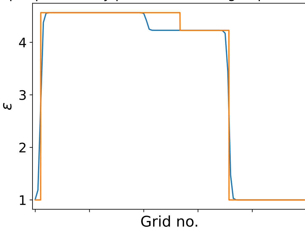
GRCWA permittivity profile. n_G = 25 , grid points = 100
